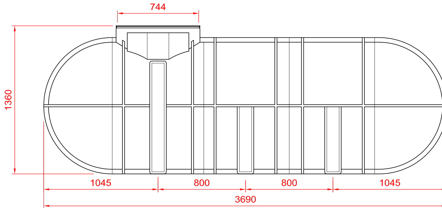
SIDE ELEVATION
