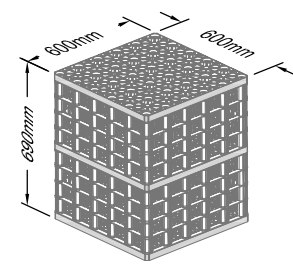
RAINSMART STM-02 DOUBLE TANK MODULE
